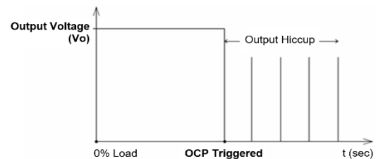
Figure 3. Hiccup at OLP/OCP
