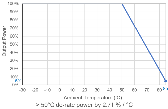
5V Standby Power De-rating Curve (Convection)
